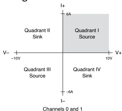
Figure 1. PXIe-4113 Quadrant Diagram
