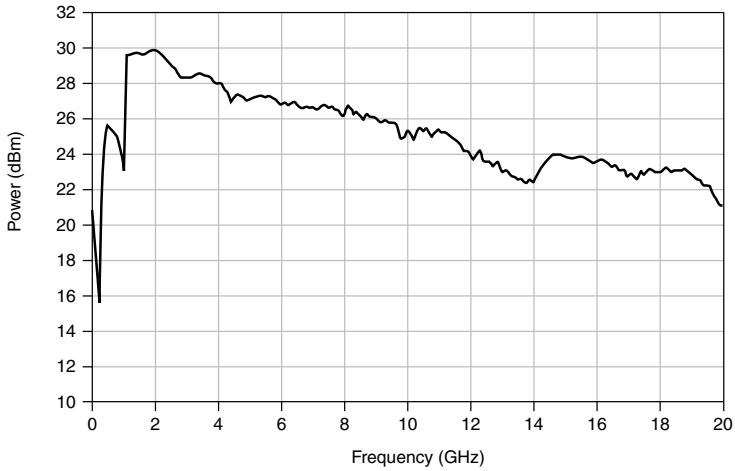
Figure 7. PXIe-5654 with PXIe-5696 Typical Maximum Available Power
