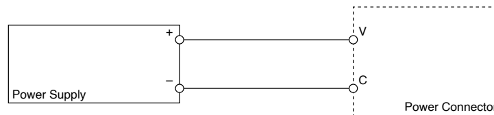
Figure 1. cRIO-9066 Power Connections
