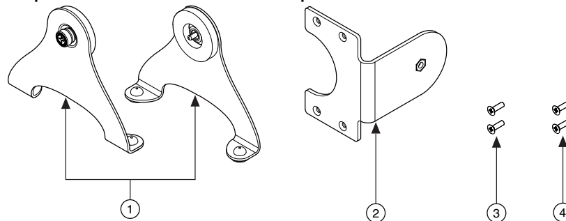
Figure 14. Components of the NI Desktop Mount Kit
