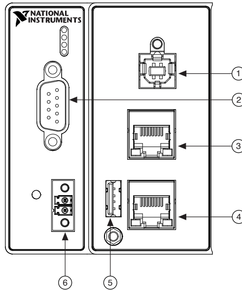
Figure 1. cRIO-9067 Ports and Connectors
