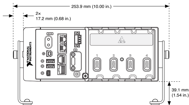
Figure 12. cRIO-9030 Desktop Mounting Front Dimensions
