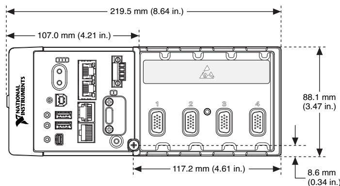
Figure 5. cRIO-9031 Front Dimensions
