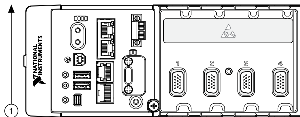
Figure 4. cRIO-9031 Horizontal Mounting
