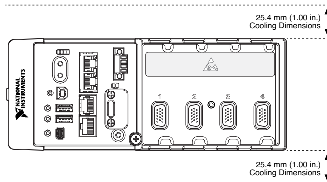
Figure 7. cRIO-9031 Cooling Dimensions
