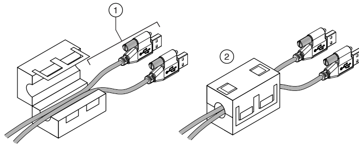
Figure 1. Installing a Ferrite on the USB Cables
