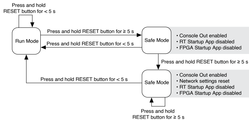
Figure 2. Reset Button Behavior
