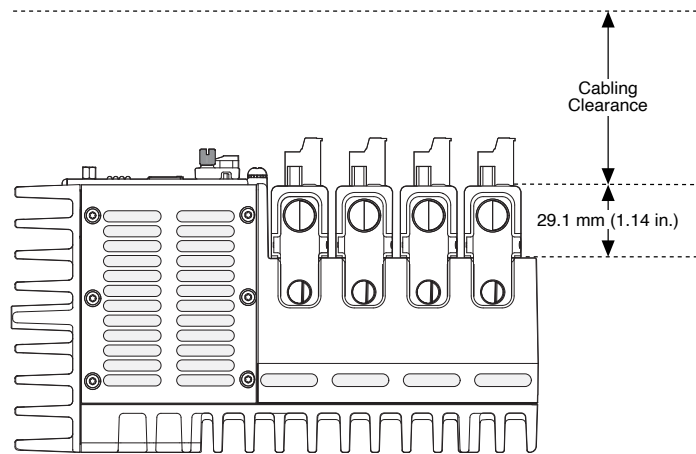
Figure 8. cRIO-9031 Cabling Clearance
