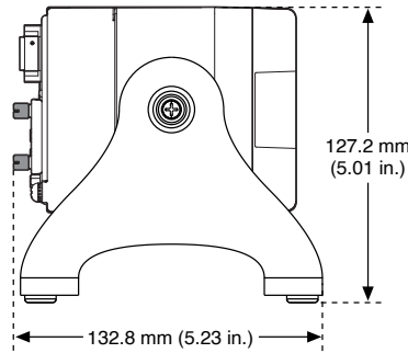
Figure 13. cRIO-9031 Desktop Mounting Side Dimensions
