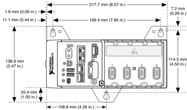
Figure 11. cRIO-9031 Panel Mounting Dimensions
