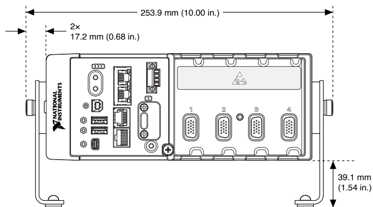
Figure 12. cRIO-9031 Desktop Mounting Front Dimensions
