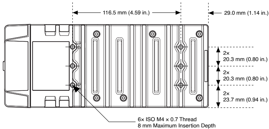
Figure 10. cRIO-9031 Surface Mounting Dimensions
