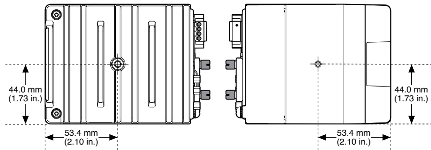
Figure 6. cRIO-9031 Side Dimensions
