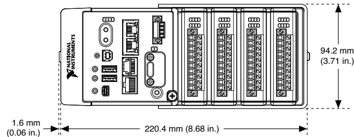
Figure 3. cRIO-9031 Module Immobilization Accessory Dimensions
