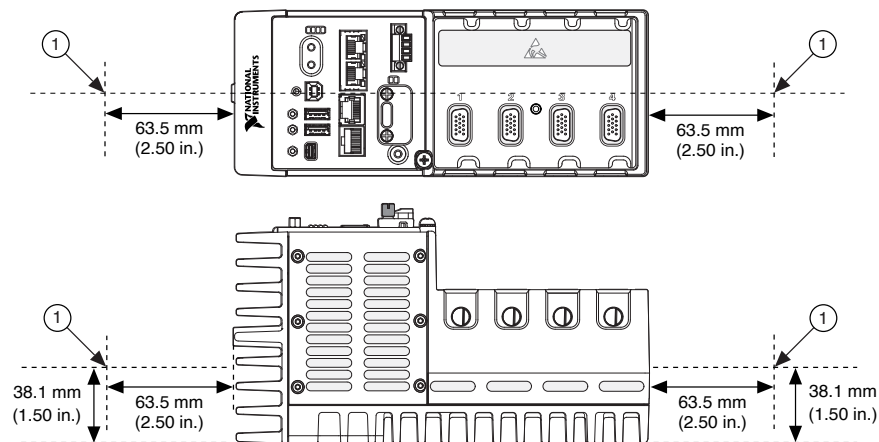
Figure 9. cRIO-9031 Ambient Temperature Location
