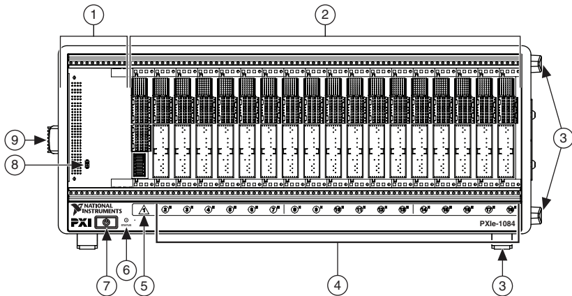
Figure 1-1. Front View of the PXIe-1084 Chassis
