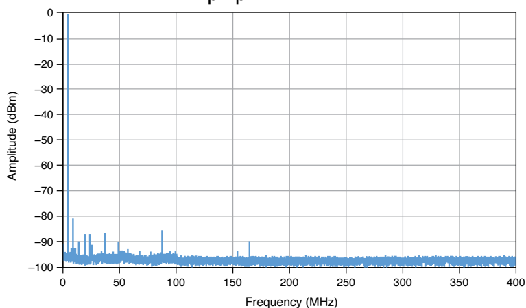
Figure 2. 5 MHz Spectrum [13] at 0.6 V_{pk-pk} , Measured
