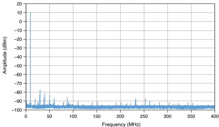
Figure 4. 1 MHz Spectrum [13] at 6.5 V pk-pk , Measured
