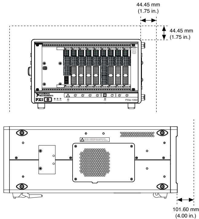
Figure 8. PXIe-1092 Cooling Clearances
