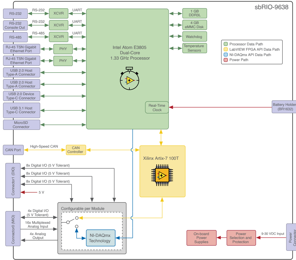
Figure 1. sbRIO-9638 Block Diagram
