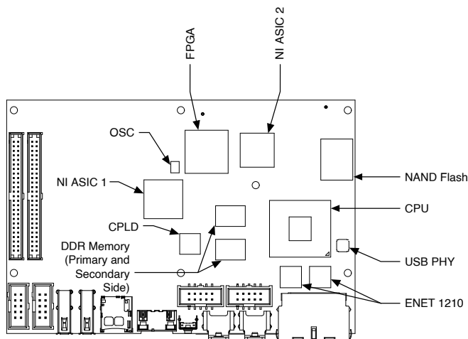
Figure 5. sbRIO-9638 Component Locations
