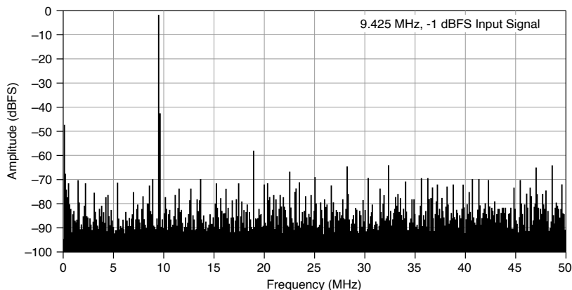
Figure 2. USB-5133 Dynamic Performance, 1 V pk-pk Range, 524,288-Point FFT, Measured
