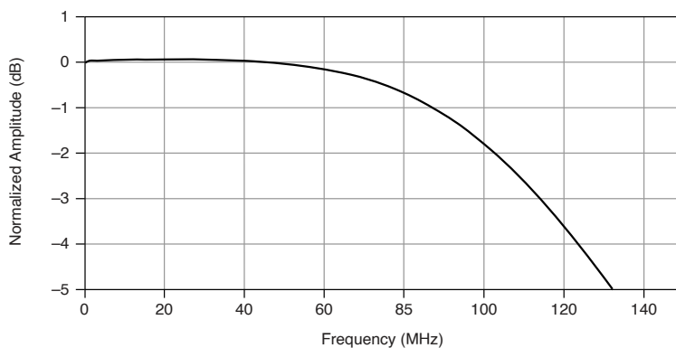
Figure 1. 50 Ω Full Bandwidth Frequency Response, 1 GS/s, 1 V pk-pk , Measured [6]
