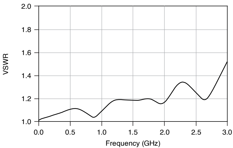
Figure 2. Channel to Common VSWR, Typical
