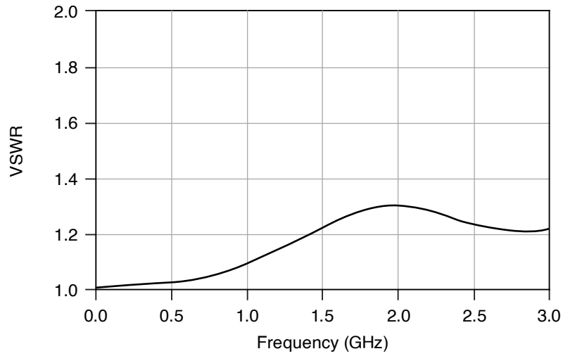
Figure 3. Termination VSWR, Typical
