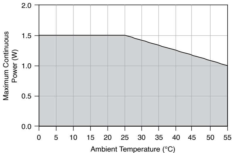
Figure 5. Termination Derating
