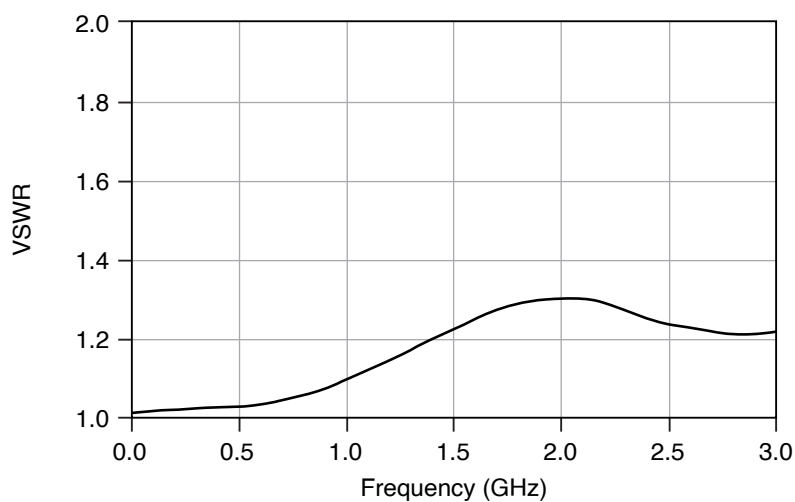
Figure 3. Termination VSWR, Typical
