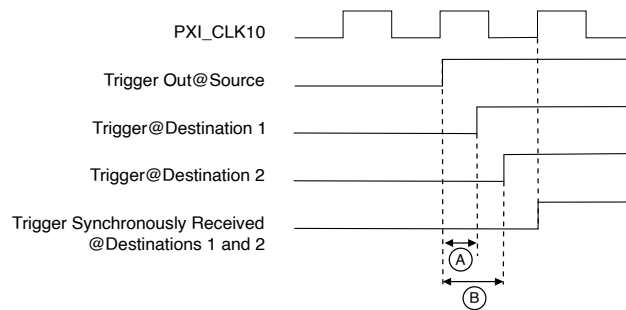
Figure 8. Synchronous Routing to Multiple Destinations
