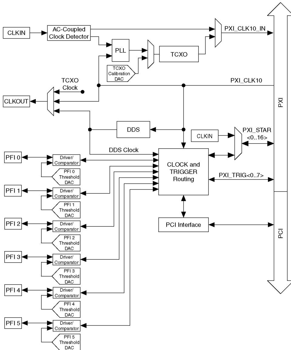
Figure 3. Functional Overview of the PXIe-6672
