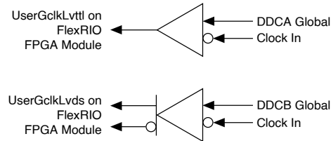
Figure 2. Clock Input (NI 6585B variant)
