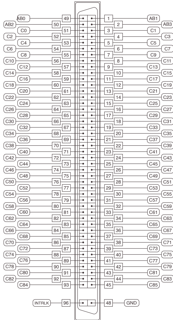
Figure 1. SWB-2815A/B Connector Pinout
