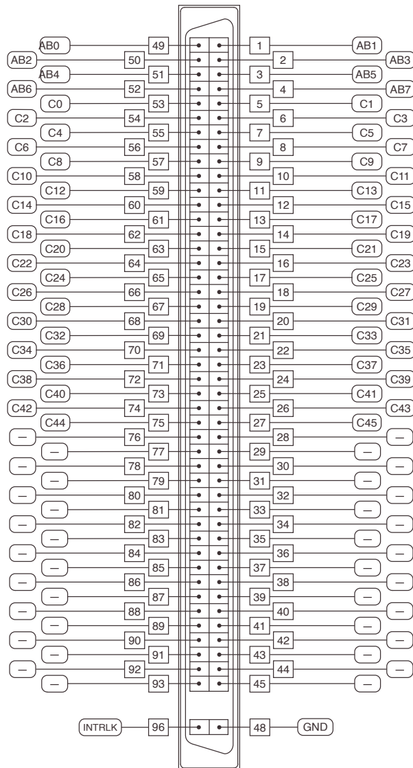
Figure 1. SWB-2816A/B Connector Pinout
