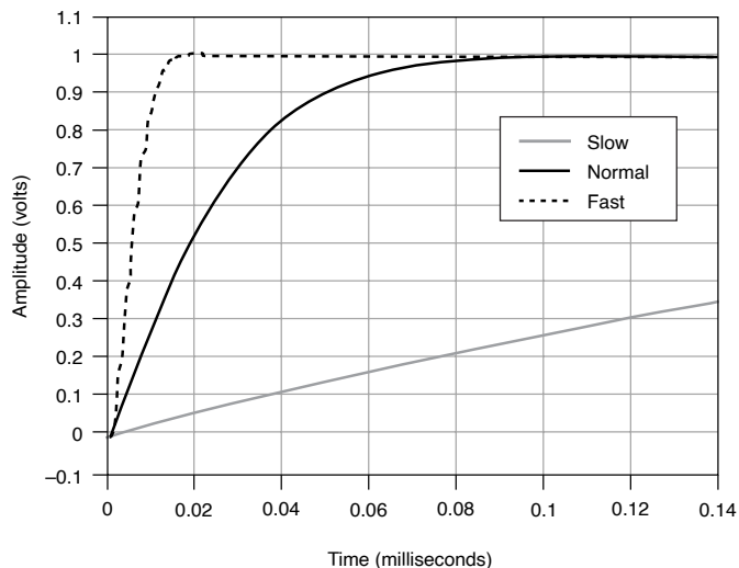
Figure 1. 1 mA Range, 100 nF Load Step Response, Typical
