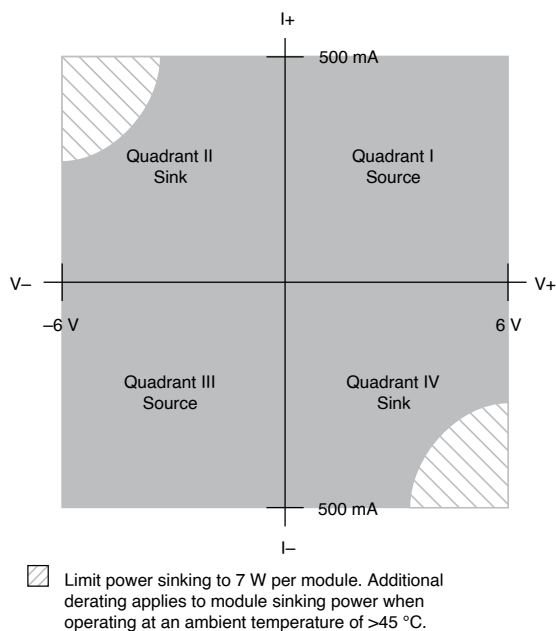
Figure 1. PXIe-4145 Quadrant Diagram, All Channels
