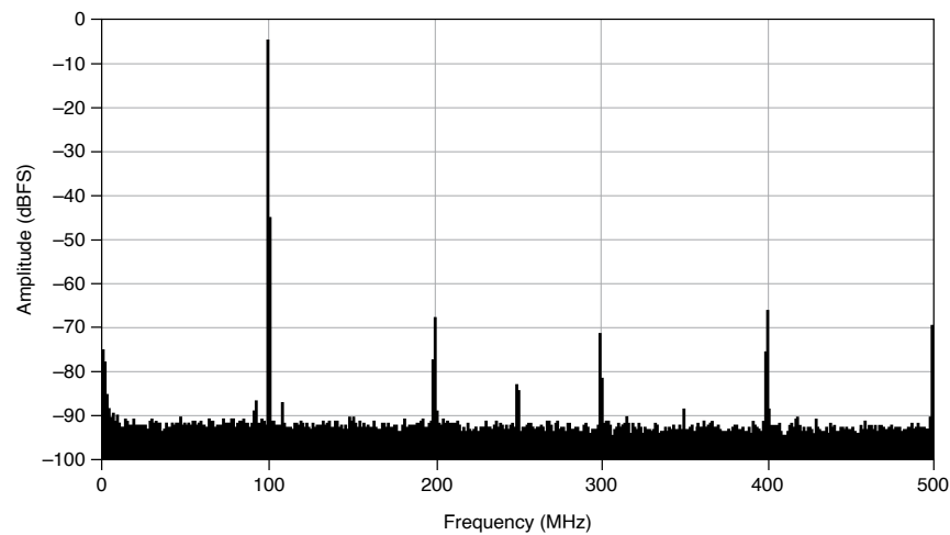
Figure 5. PXI-5153 TIS Dynamic Performance, 2 V_{pk-pk} Input Range, 100 MHz Input Signal, Measured
