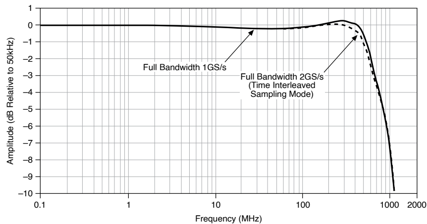
Figure 2. PXI-5153 Frequency Response, 5 V pk-pk through 0.1 V pk-pk Input Ranges, Measured
