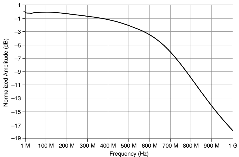
Figure 4. PXIe-5160 1 M \Omega Frequency Response, 1 V pk-pk , Measured [18]
