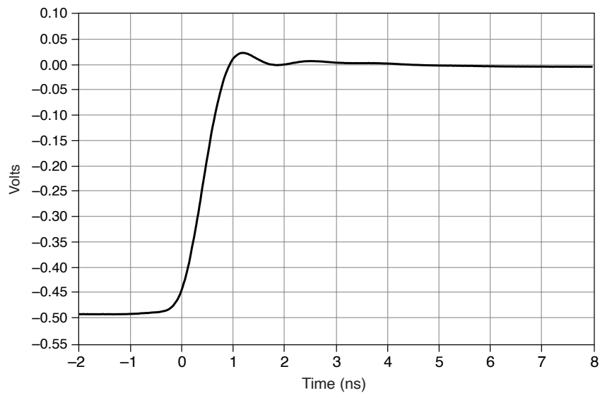
Figure 2. PXIe-5160 Step Response, 1 M \Omega , 1 V pk-pk Input Range, -0.25 V Programmable Offset, 500 ps Rising Edge, Measured [17]
