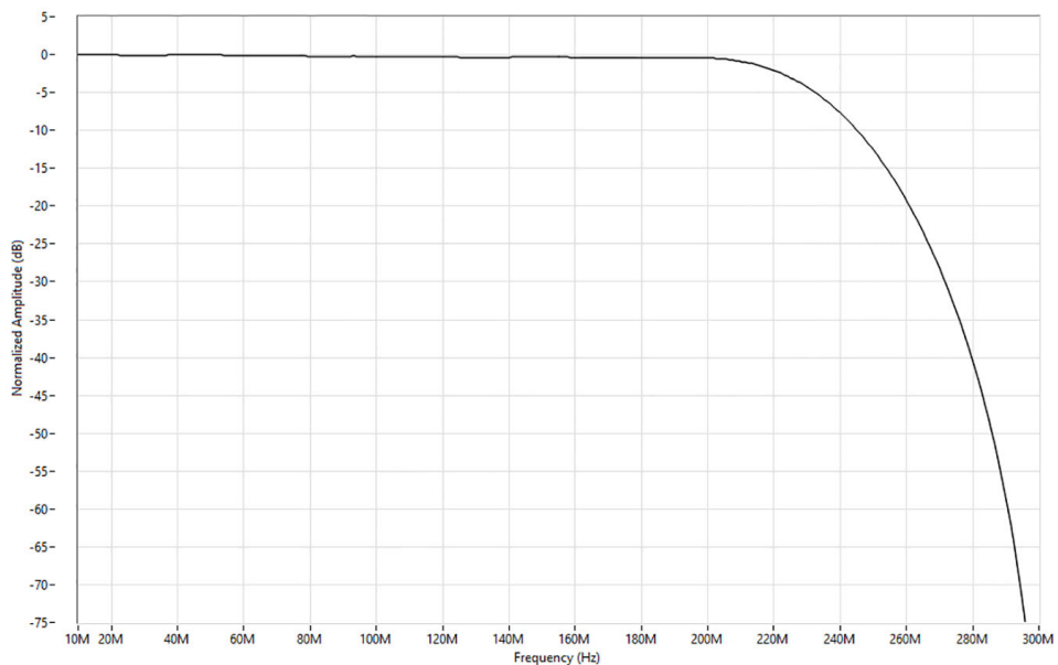
Figure 8. DC-Coupled Frequency Response Zoomed In, Measured
