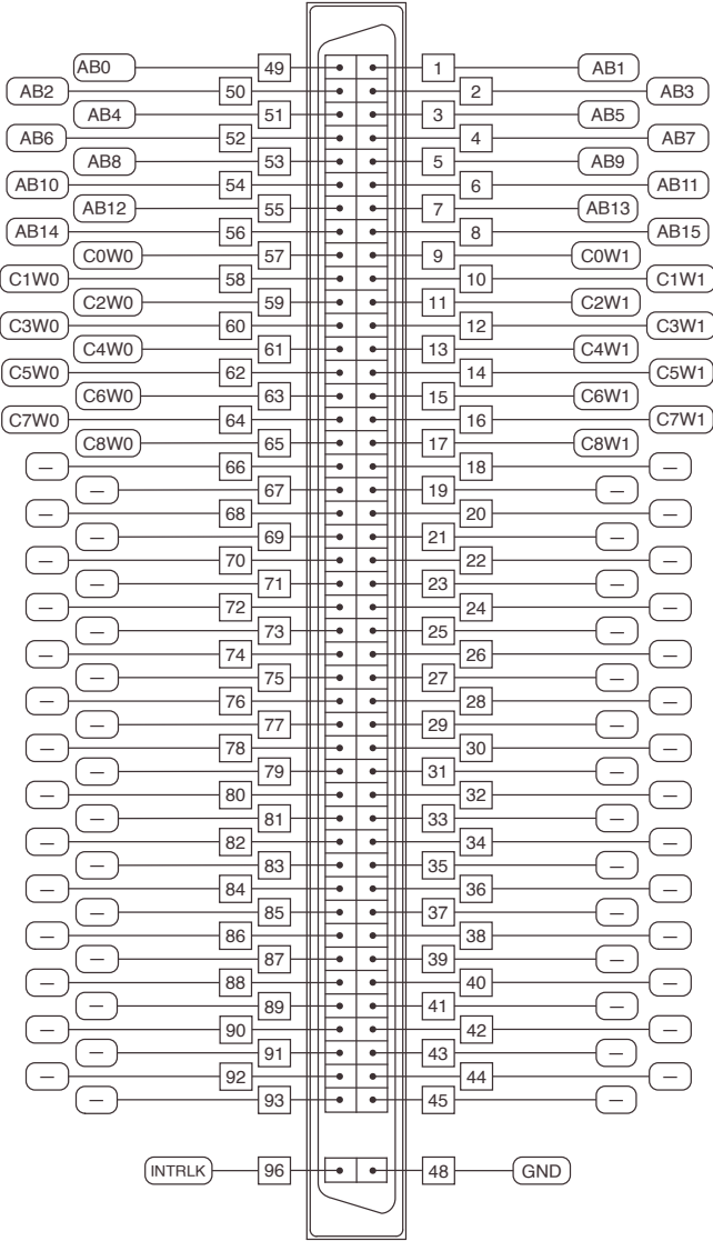
Figure 1. NI 2814A/B Connector Pinout
