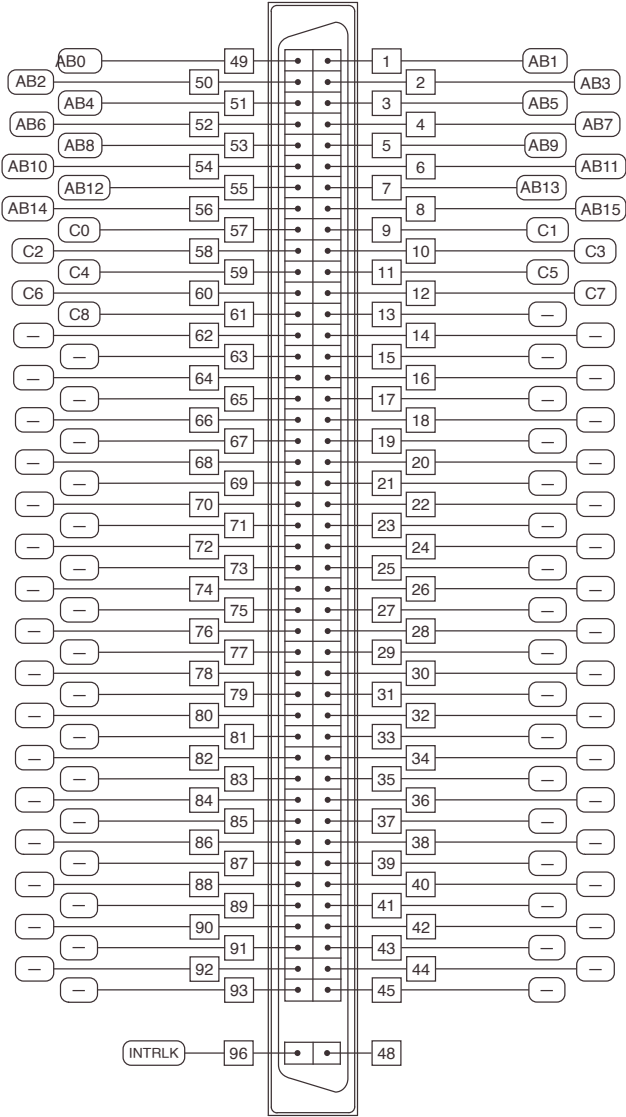
Figure 1. SWB-2812A/B Connector Pinout
