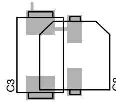
Figure 12. Option to Place an Electrolytic or Tantalum Capacitor
