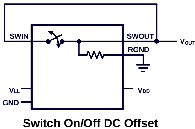
Figure 4: Test Circuit 3
