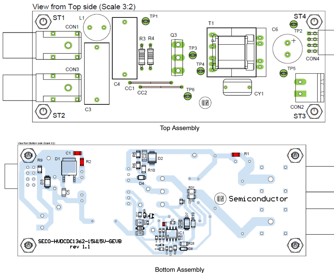
Figure 22. Layout
