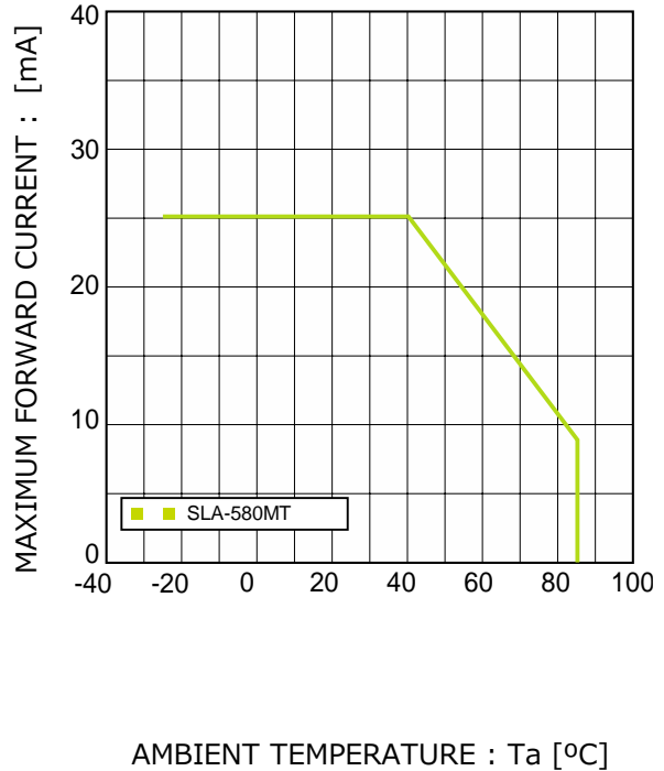
Fig.4 Derating
