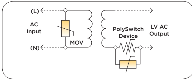
Figure 5. A coordinated protection scheme for Class 2 power sources.
