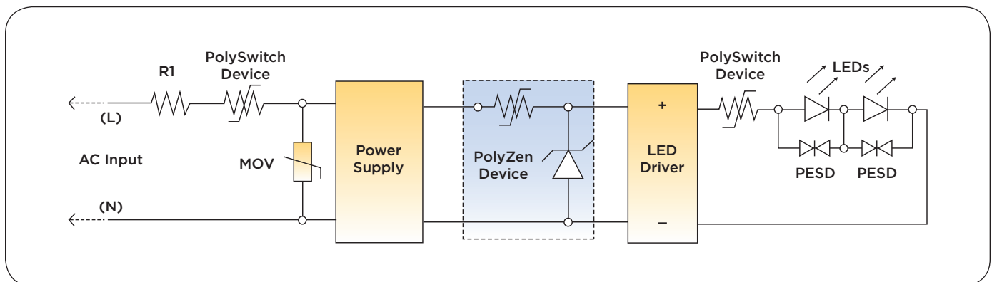
Figure 4. Coordinated protection scheme for LED Driver inputs and outputs.
