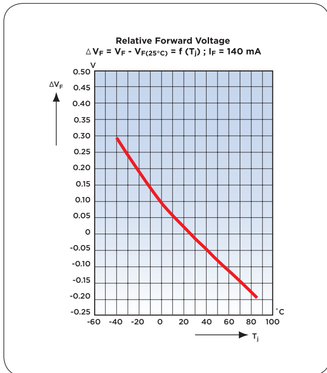
Figure 2. Forward voltage drops as junction temperature rises.
