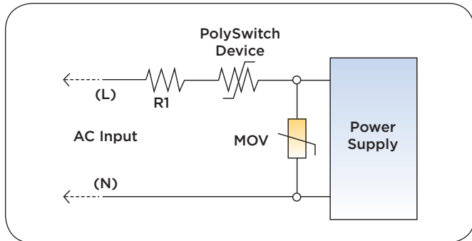
Figure 3. Typical circuit protection design for switch-mode power supplies.
