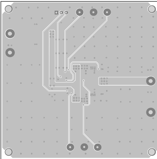
Figure 6: Mid-Layer 2
