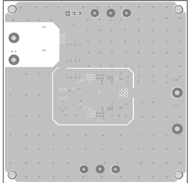
Figure 5: Mid-Layer 1
