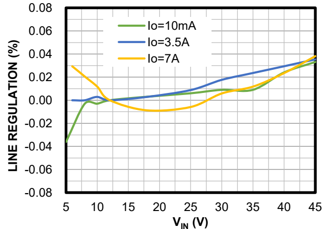
Line Regulation
