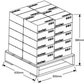
Current Box 309073001 289 X 270 X 95 (L, W, D in mm) Box holds 950pcs
