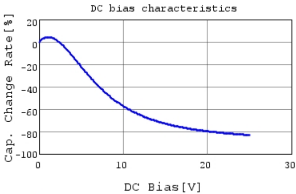
GRM31CR71E106KA12 C-DC bias capchange, 25.0c
