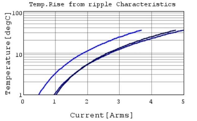
GRM31CR71E106KA12 Temp.rise — 80kHz
