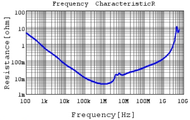
GRM31CR71E106KA12 R DCOV,25degC
