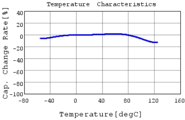
GRM31CR71E106KA12 C-Temp. capchange, DC0.0V,
