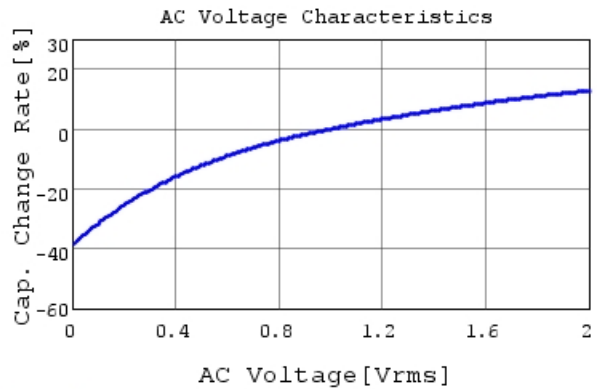
GRM31CR71E106KA12 C-AC Voltage capchange, Dc
