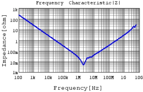
GRM31CR71E106KA12 |Z| DCOV,25degC
