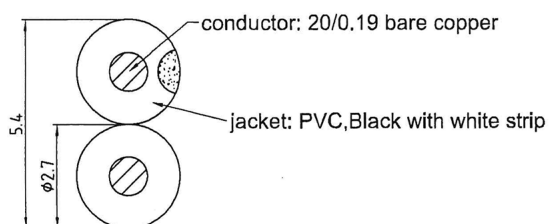
Cable Construction
