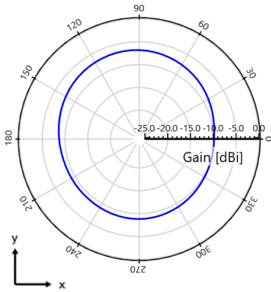
High Band measured at 315 MHz
