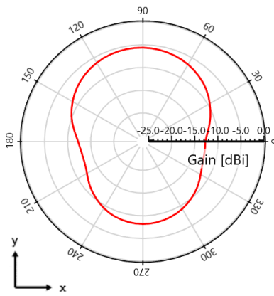
High Band measured at 400 MHz
