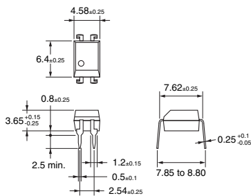
PCB Terminals Weight: 0.25 g
