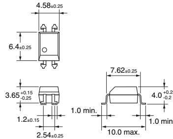
Surface-mounting Terminals Weight: 0.25 g
