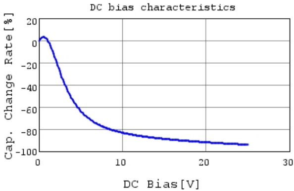
GRM155R61E105KA12 C-DC bias capchange, 25.0c
