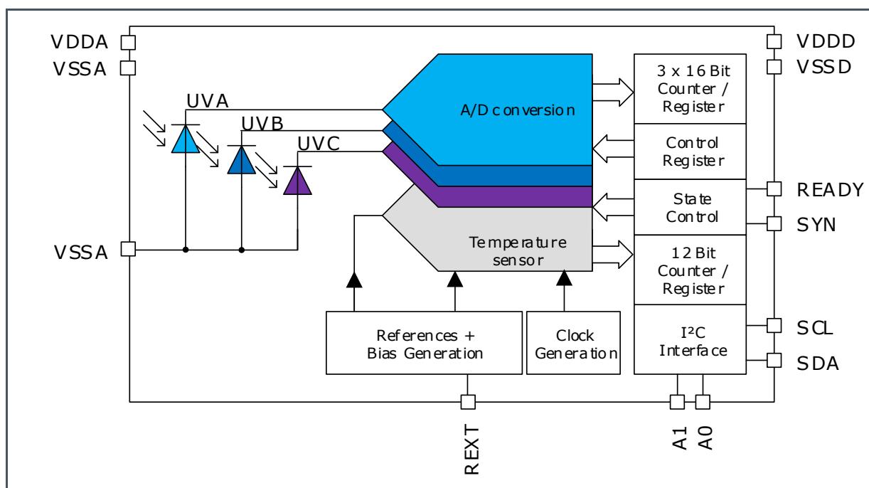
Figure 2: Functional Blocks of the AS7331
