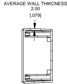
SECTION A-A SCALE 3 / 8
