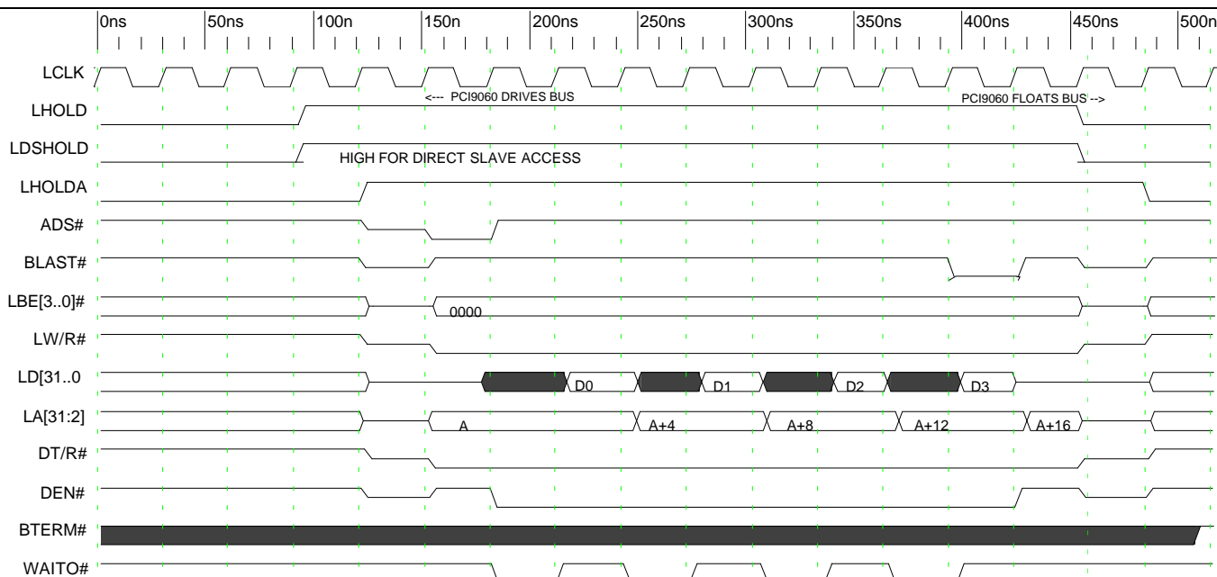
Timing Diagram 16. (CX Mode) Burst Read from Local Bus (1 Wait State Programmed)
