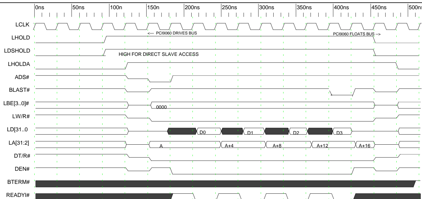
Timing Diagram 15. (CX Mode) Direct Slave or DMA Burst Read from Local Bus (1 Wait State)
