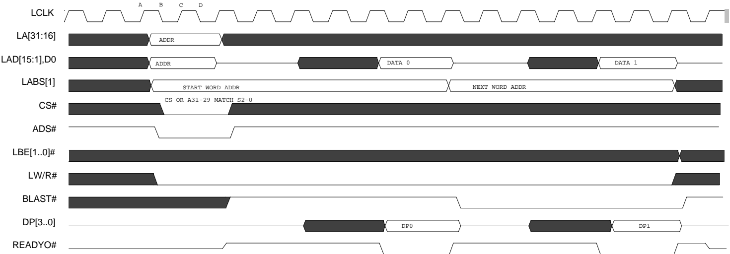
Timing Diagram 31. (SX Mode) Local Bus Read from Configuration Register
