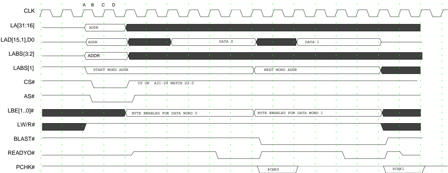
Timing Diagram 30. (SX Mode) Local Bus Write to Configuration Register
