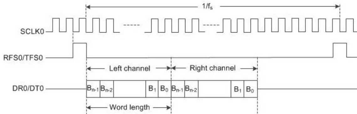
Figure 2-11. Timing Diagram for PCM Modes (Master/Slave)
