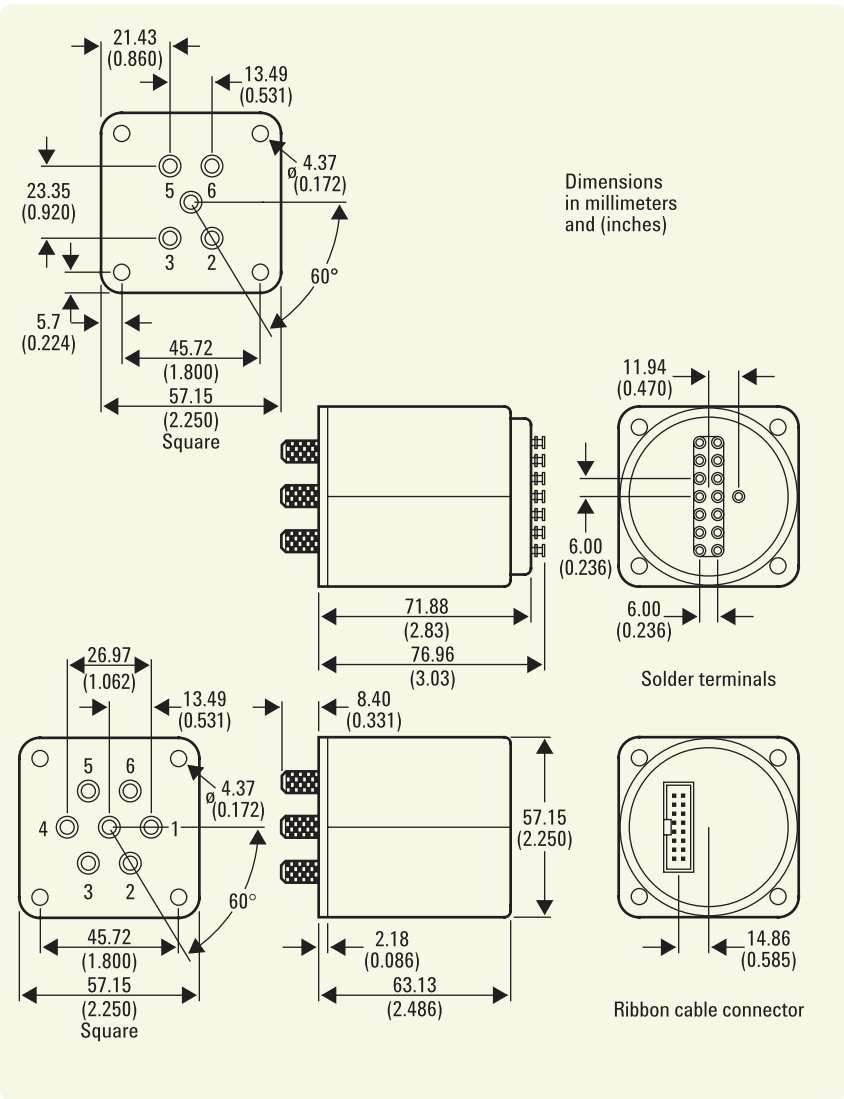
Figure 14. Product dimensions for L7104/106 A,B,C and L7204/206 A,B,C
