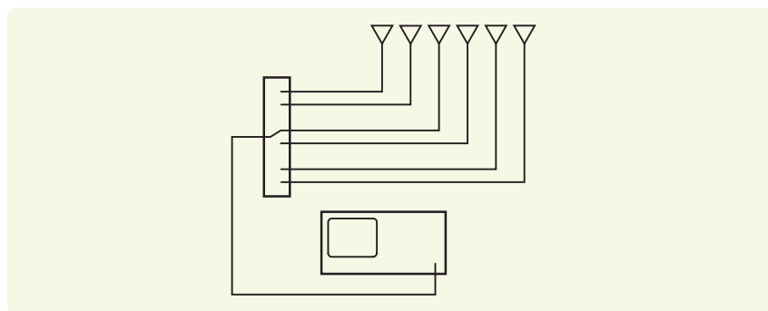
Figure 4. Multiport matrix
