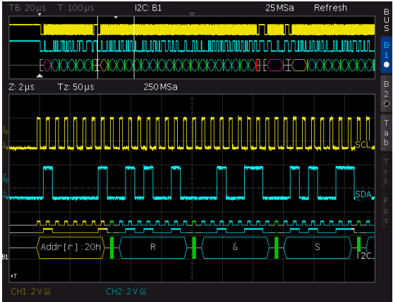
Gather insight into the digital communications on your circuitry
