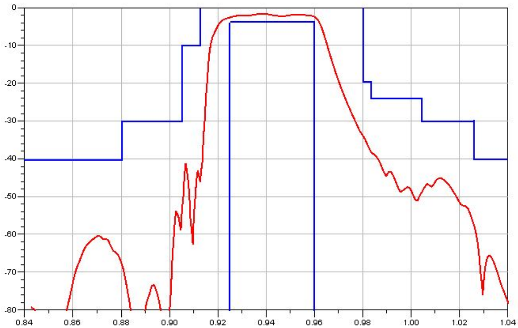
Frequency Response
