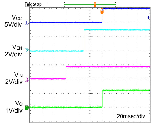
Figure.37 Start-up Sequence 5 (VIN → VEN → VCC) Ta=105°C
