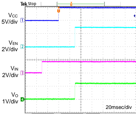
Figure.34 Start-up Sequence 4 (VIN → VCC → VEN) Ta=105°C
