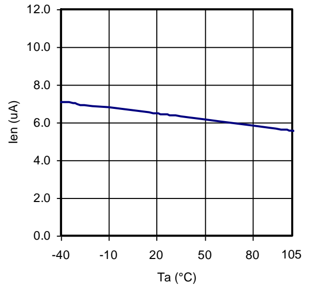
Figure.51 Ta-IEN
