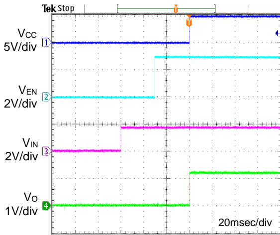
Figure.36 Start-up Sequence 5 (VIN → VEN → VCC) Ta=25°C
