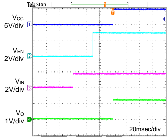
Figure.35 Start-up Sequence 5 (VIN → VEN → VCC) Ta=-40°C
