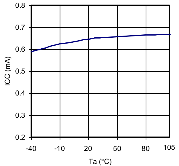
Figure.45 T_a - I_{cc}
