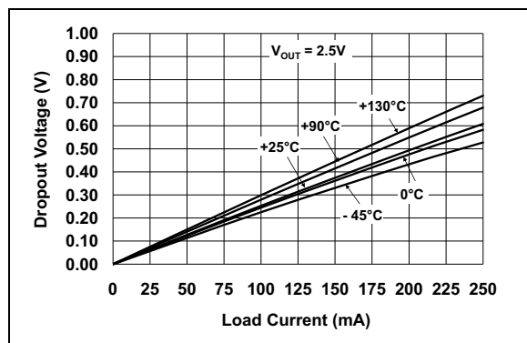
FIGURE 2-14: Dropout Voltage vs. Load Current.
