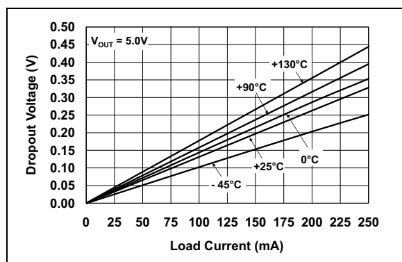
FIGURE 2-15: Dropout Voltage vs. Load Current.
