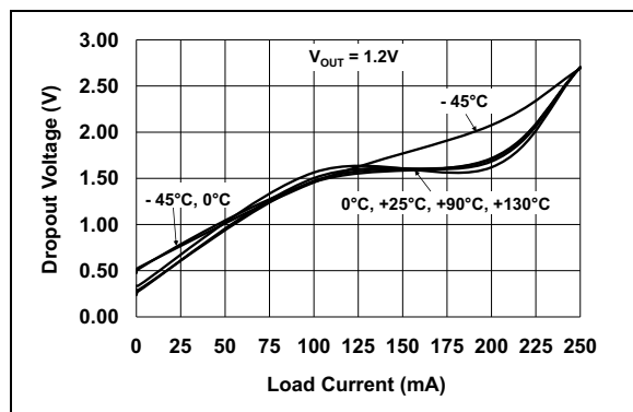
FIGURE 2-13: Dropout Voltage vs. Load Current.
