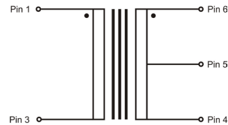
Electrical Schematic VTX-101-16##
