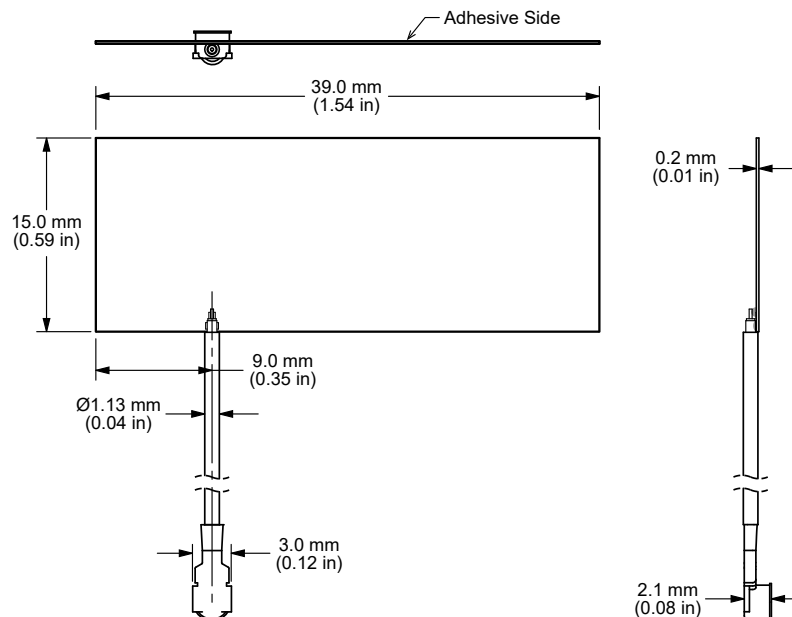
Figure 1: ANT-8/9-FPC-UFL Dimensions
