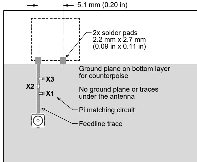
Figure 10. nanoSplatrch Placement on PCB
