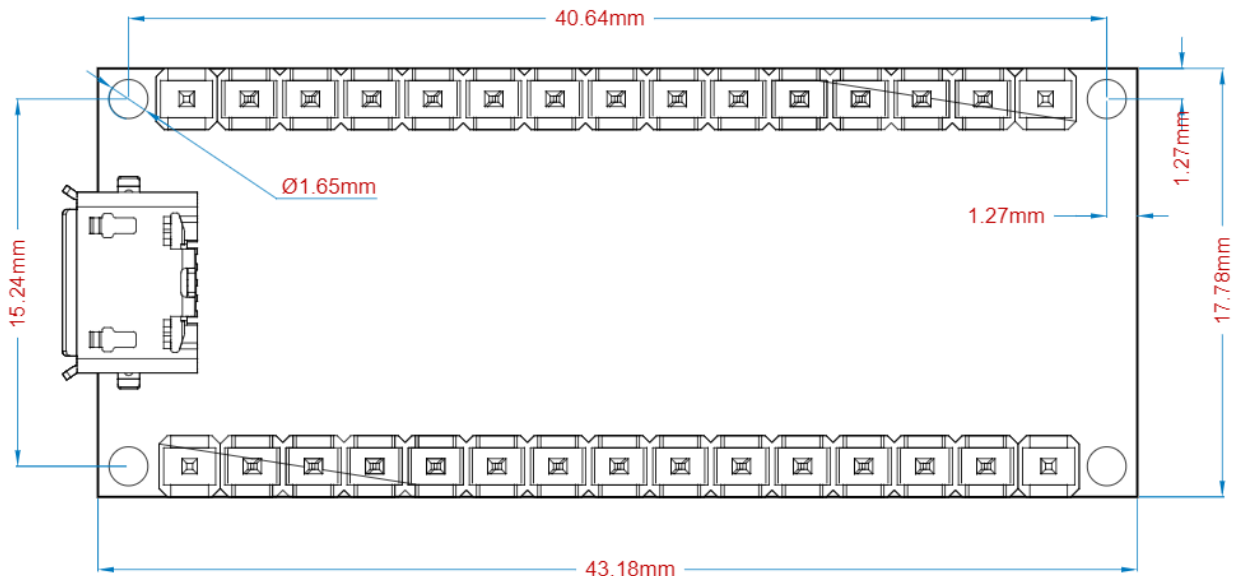
Board layout
