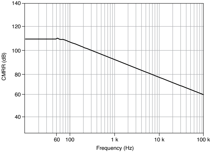
Figure 2. AI CMRR
