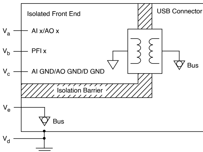
Figure 5. USB-6216 Safety Voltages
